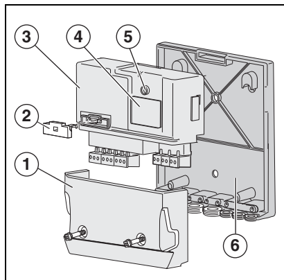
Fig. 1 Overview EM10
